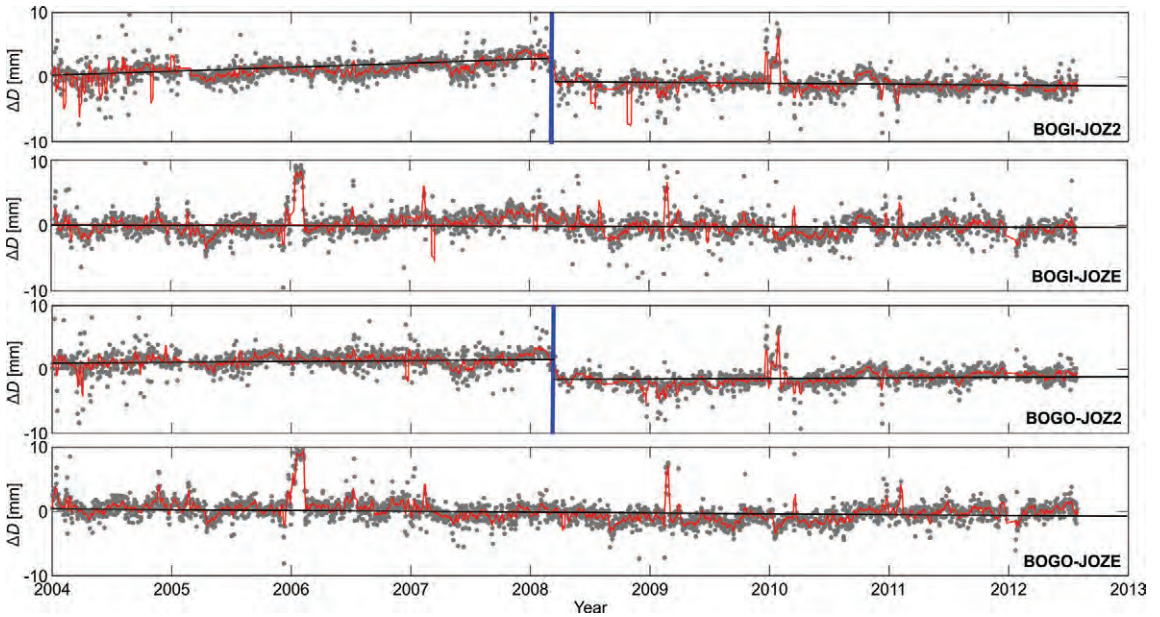
Fig. 5. Variations in baseline lengths; daily solutions (grey dots) and 7-day average solutions (red line); linear trends (black line); blue vertical lines represent the period of antenna replacement at JOZ2
