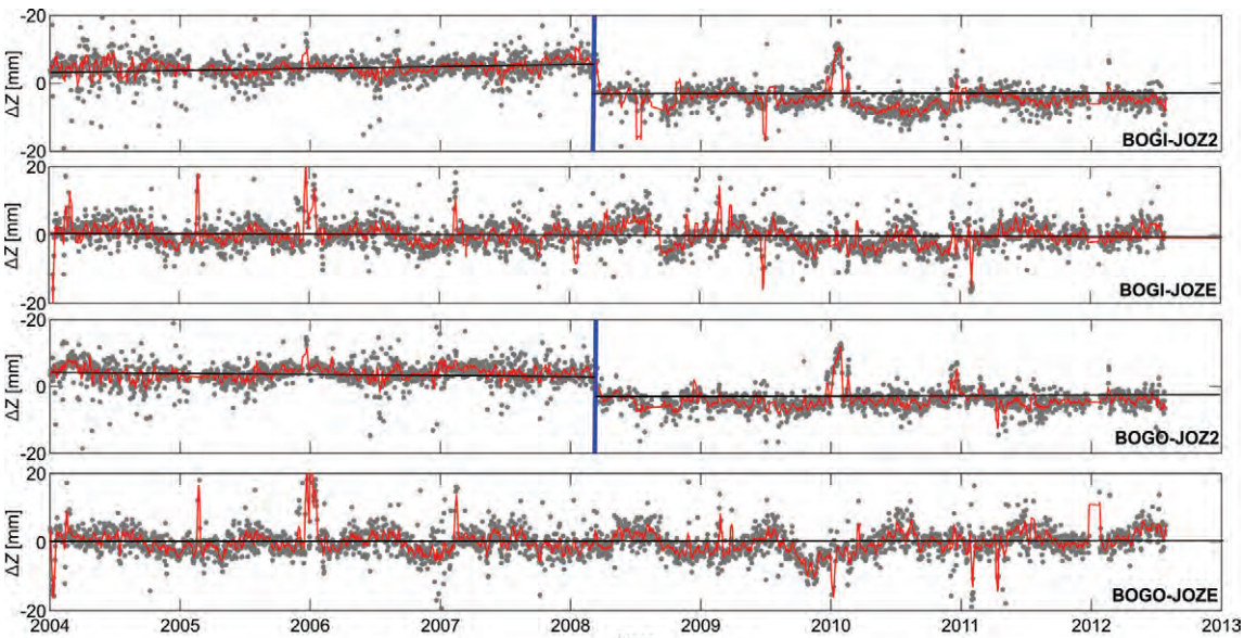
Fig. 4. Variations in Z-component; daily solutions (grey dots) and 7-day average solutions (red line); linear trends (black line); blue vertical lines represent the period of antenna replacement at JOZ2
