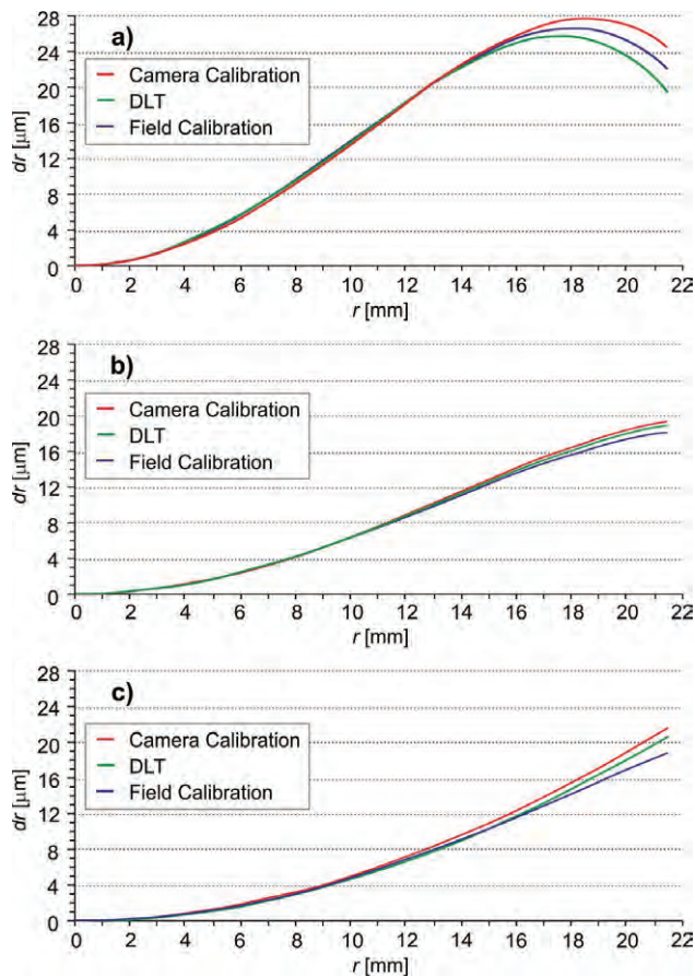
Fig. 5. Radial distortion of 25 mm lens a), 35 mm lens b) and 50 mm lens c) for three calibration methods applied
