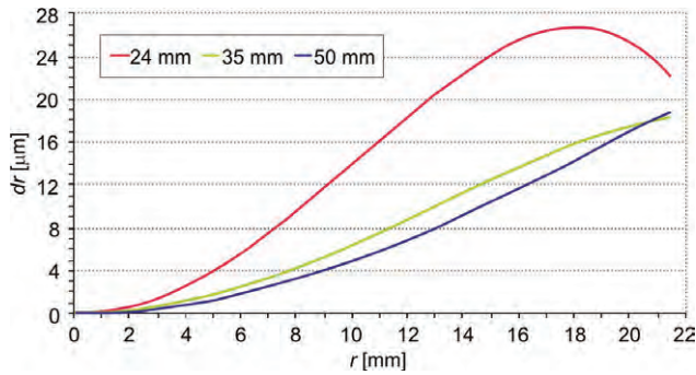
Fig. 4. Radial distortion of tested lenses obtained from the calibration using 3D test field
