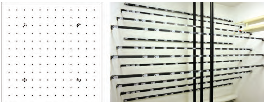
Fig. 2. 2D test field (left) and 3D test field (right)
