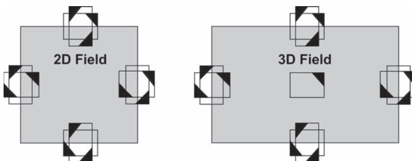
Fig. 3. Images configurations for calibration in PhotoModeler for 2D field (left) and 3D field (right)
